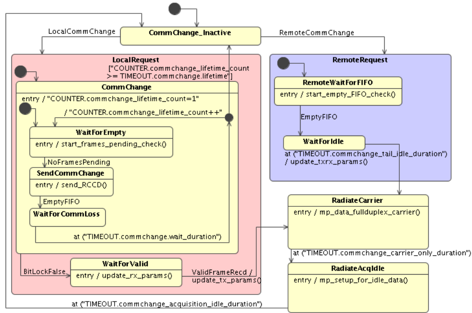
Figure 4. Proximity-1 Communications Change statechart, composed of 12 states, 17 transitions, and 8 actions.
