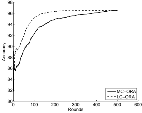
Figure 3. Active example selection (LC) paired with oracle labeling learns more quickly than MC paired with an oracle. Results shown use classifier LOG.
